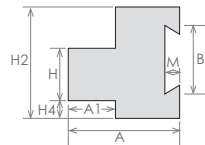
Tool Block
